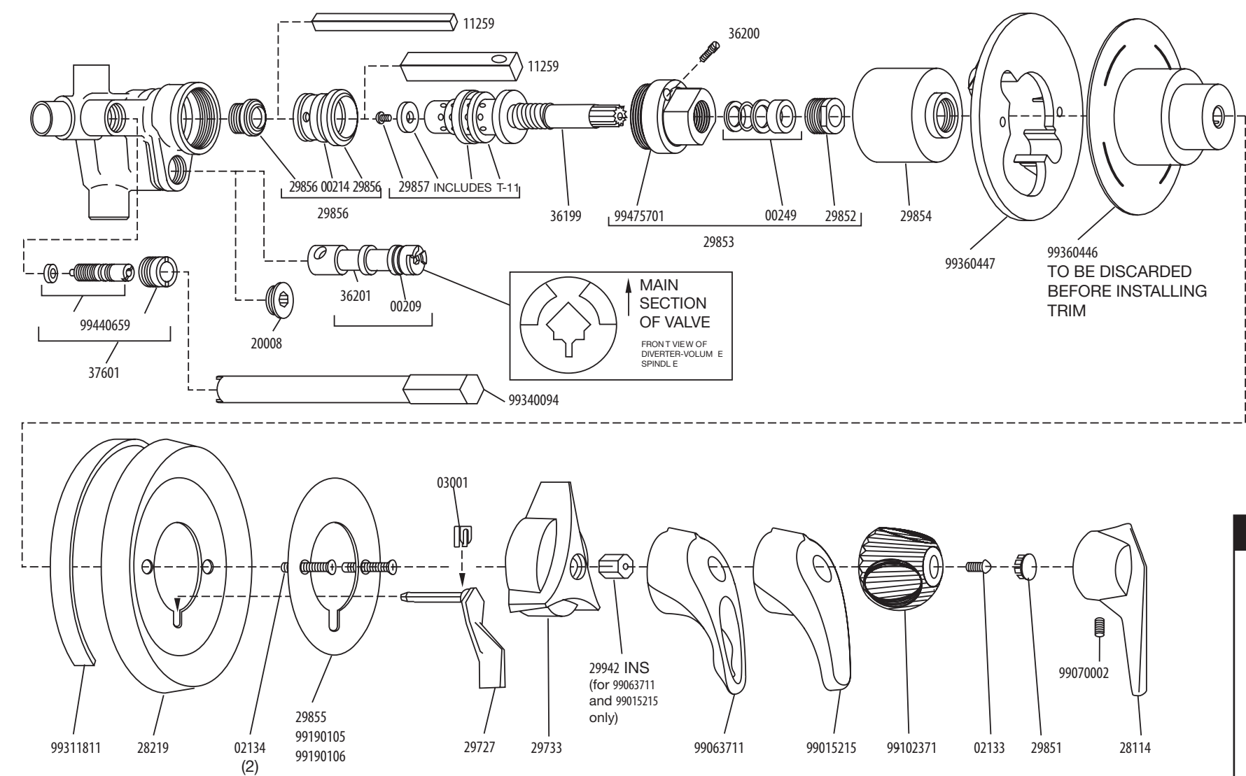
FIGURE 9 Parts Breakdown
